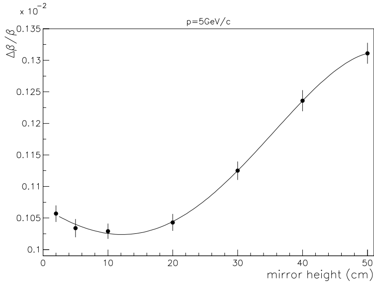
Figure 13: Distributions of \Delta\beta/\beta as a function of the height of the cone mirror in geometry b).
