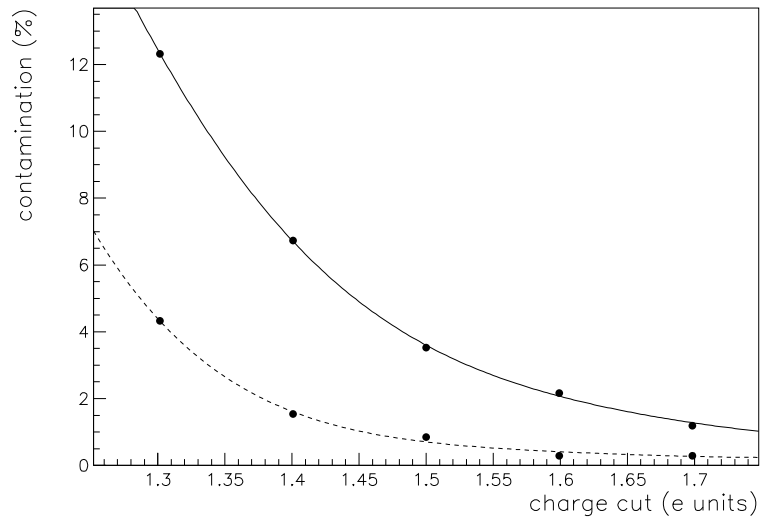
Figure 21: Contamination of protons in a sample of helium for a ratio of fluxes 7:1, as a function of the cut, if a) all photon hits are used, and b) only unscattered photons are counted.
