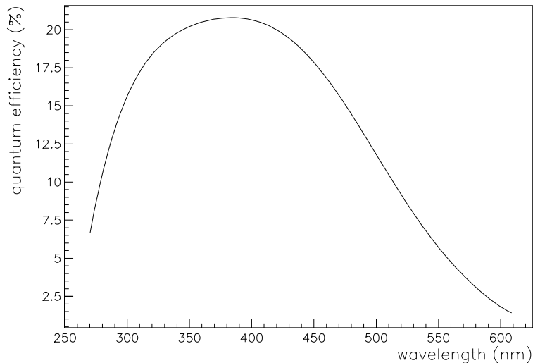
Figure 3: Quantum efficiency of the Hamamatsu 5900 photomultiplier with bialkali photocathode and a borosilicate glass window.
