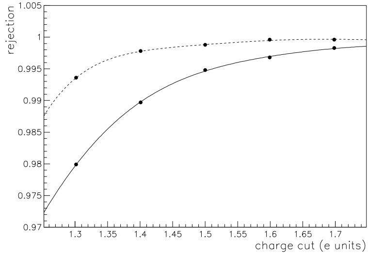
Figure 20: Rejection curves for p/He separation if all photon hits are used (solid line); if only unscattered photons are counted (dashed curve).
