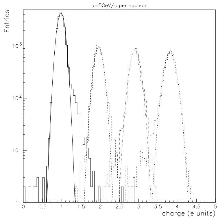
Figure 18: Distribution of z for nuclei with z < 5 and momentum 5 GeV/c per nucleon, for geometry b).
