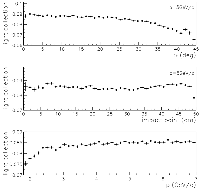
Figure 6: Light collection efficiency as a function of a) incident angle, b) impact point and c) momentum.
