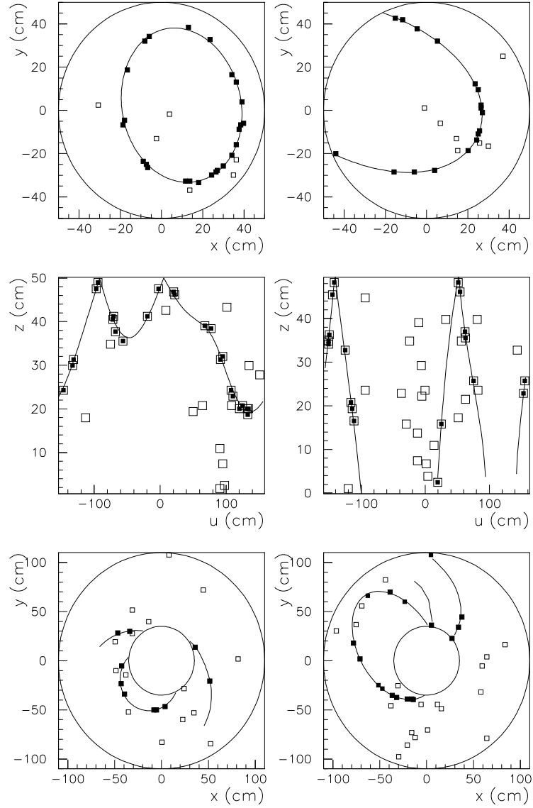
Figure 5: Display of patterns of hits for geometries a) (top row), b) (middle row) and c) (bottom row). The solid points represent the hits selected by the pattern recognition. The curves resulted from the fit to the set of selected hits. In geometry b) the variable u = R \tan^{-1}(y/x) , where R is the radius of the cylinder and (x, y) the coordinates of the hit point. Each plot displays one event only. As can be seen, the rings are highly dependent on the kinematics of the incident particle, specially for the latter two geometries.
