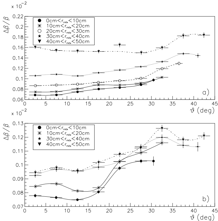
Figure 12: Distributions of \Delta\beta/\beta as a function of polar angle of the incident particle, for geometries b) (top) and c).
