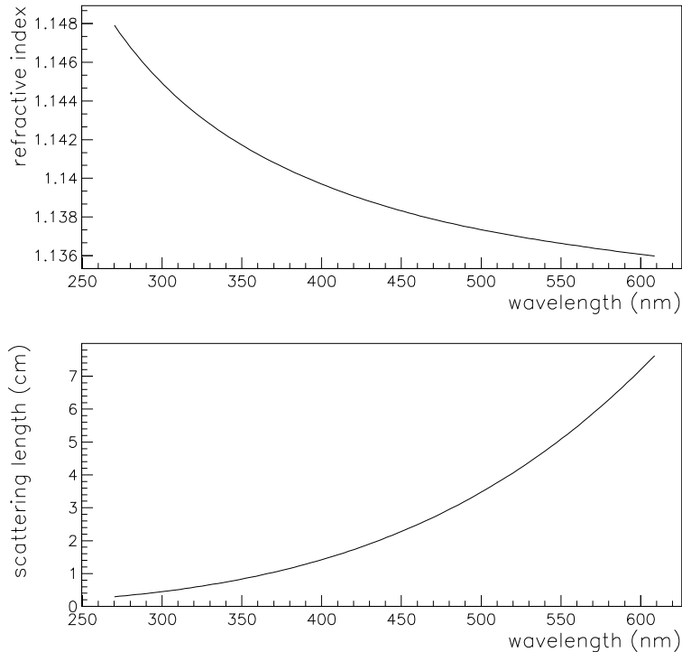
Figure 2: Optical properties of aerogel as a function of the wavelength: a) refractive index, scaled from the optical dispersion of fused silica and b) the Rayleigh scattering length for an aerogel with a clarity coefficient C = 0.018\mu\text{m}^4/\text{cm} .
