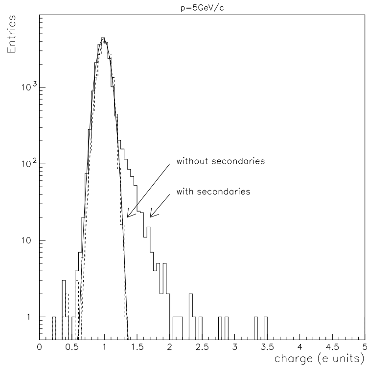
Figure 17: Distribution of z for 5 GeV/c protons with an angular distribution given by the acceptance of the detector: all effects included (solid line); production of secondary particles or \delta -rays suppressed (dashed line).
