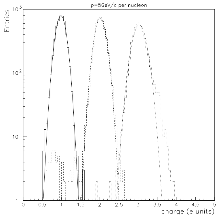
Figure 19: Distribution of z for nuclei with z < 5 and momentum 5 GeV/c per nucleon if only pattern selected photons are used to determine the charge, for geometry b).
