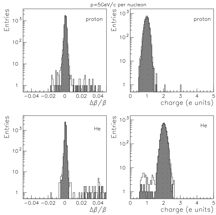
Figure 22: Distributions of \Delta\beta/\beta and z for protons and He. The hatched areas are for events with more than 3% CL.
