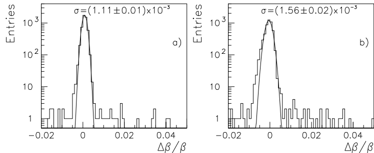
Figure 16: Distributions of \Delta\beta/\beta for a proximity focused geometry using a) the fit method discussed in this work and b) the average \theta_c method.
