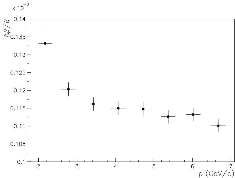
Figure 10: Distribution of \Delta\beta/\beta , for geometries b) and c) (at right), for a pixel size of 7 \times 7\text{mm}^2 , upon application of the pattern recognition.
