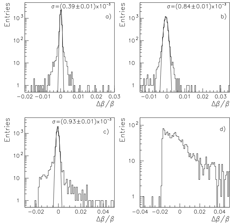
Figure 7: Contribution of different physics processes to \Delta\beta/\beta . a) "pure signal" , i.e.. no optical dispersion, no \delta -rays, no Rayleigh scattering; b) as a) plus the effect of the chromatic dispersion; c) as b) plus the inclusion of physical processes yielding secondary particles in the radiator; d) all physical effects (chromaticity, Rayleigh scattering and production of photoelectrons by secondary particles) are included. These curves refer to geometry c). Results are similar for the other geometries considered. No pattern recognition is applied.
