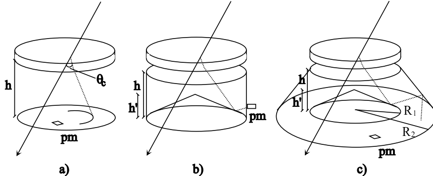
Figure 1: Geometries of the detectors considered: a) proximity focused, b) derived from a) with a conical mirror and photodetectors on the lateral wall of a cylinder, and c) a double conical mirror assembly with readout at the lowest plane.
