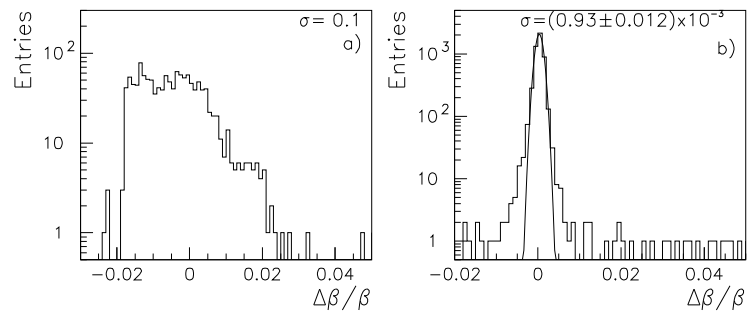
Figure 15: \Delta\beta/\beta , for an aerogel radiator of clarity coefficient C = 0.01\mu\text{m}^4/\text{cm} , and geometry b), when all effects are included, a) without and b) with pattern recognition.
