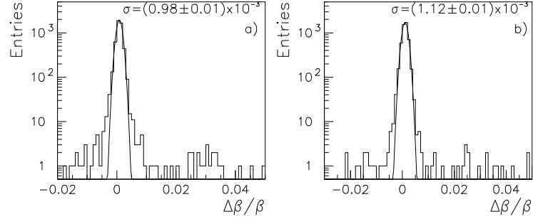
Figure 8: Distribution of \Delta\beta/\beta , for geometries b) and c) (at right), upon application of the pattern recognition. The background influence is highly reduced.
