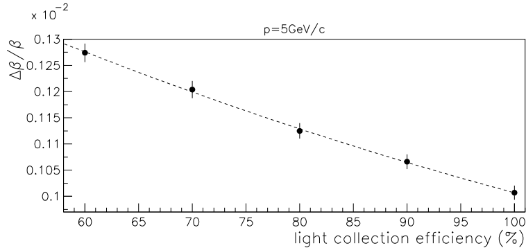
Figure 14: The resolution \Delta\beta/\beta as a function of the light collection efficiency.
