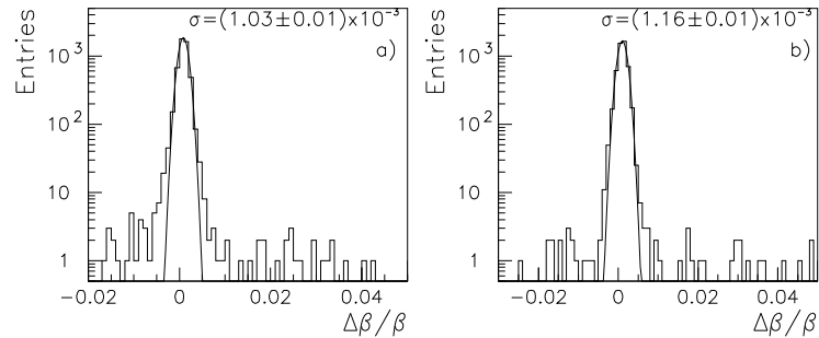
Figure 10: Distribution of \Delta\beta/\beta , for geometries b) and c) (at right), for a pixel size of 7 \times 7\text{mm}^2 , upon application of the pattern recognition.
