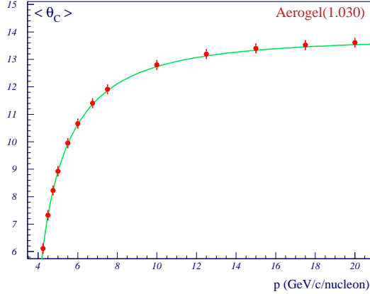
Figure 5. Čerenkov angle reconstructed as function of particle momentum for an aerogel radiator.
