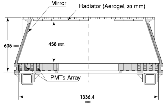
Figure 2. The RICH detector.
