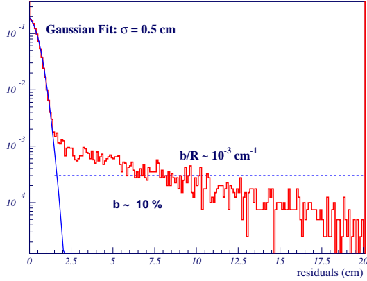
Figure 3. Distribution of the hit residuals with respect to the expected Čerenkov pattern.
