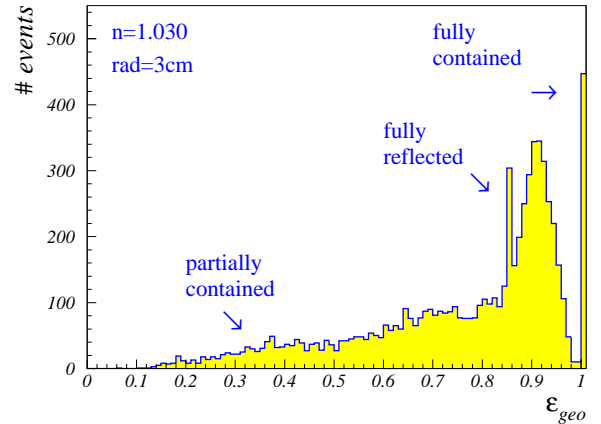
Figure 6. Photon geometrical acceptance for events in the RICH detector.
