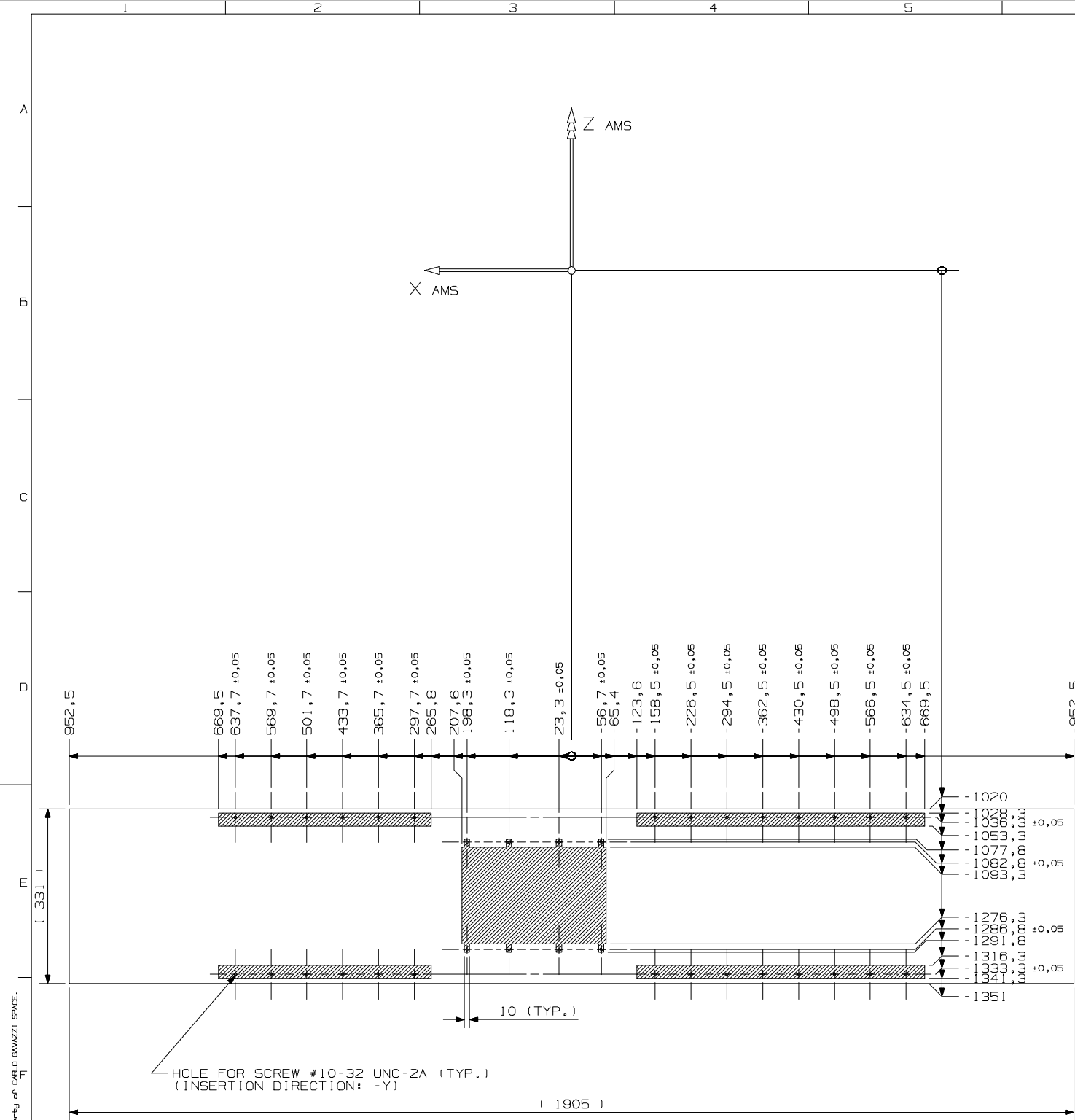
RAM RADIATOR
